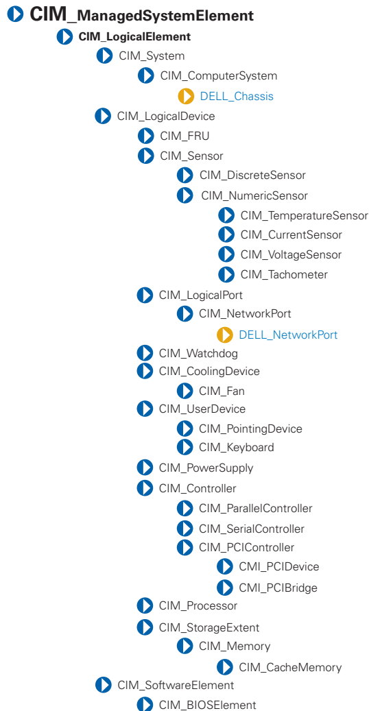
Figure 3-1. CIM_LogicalElement
